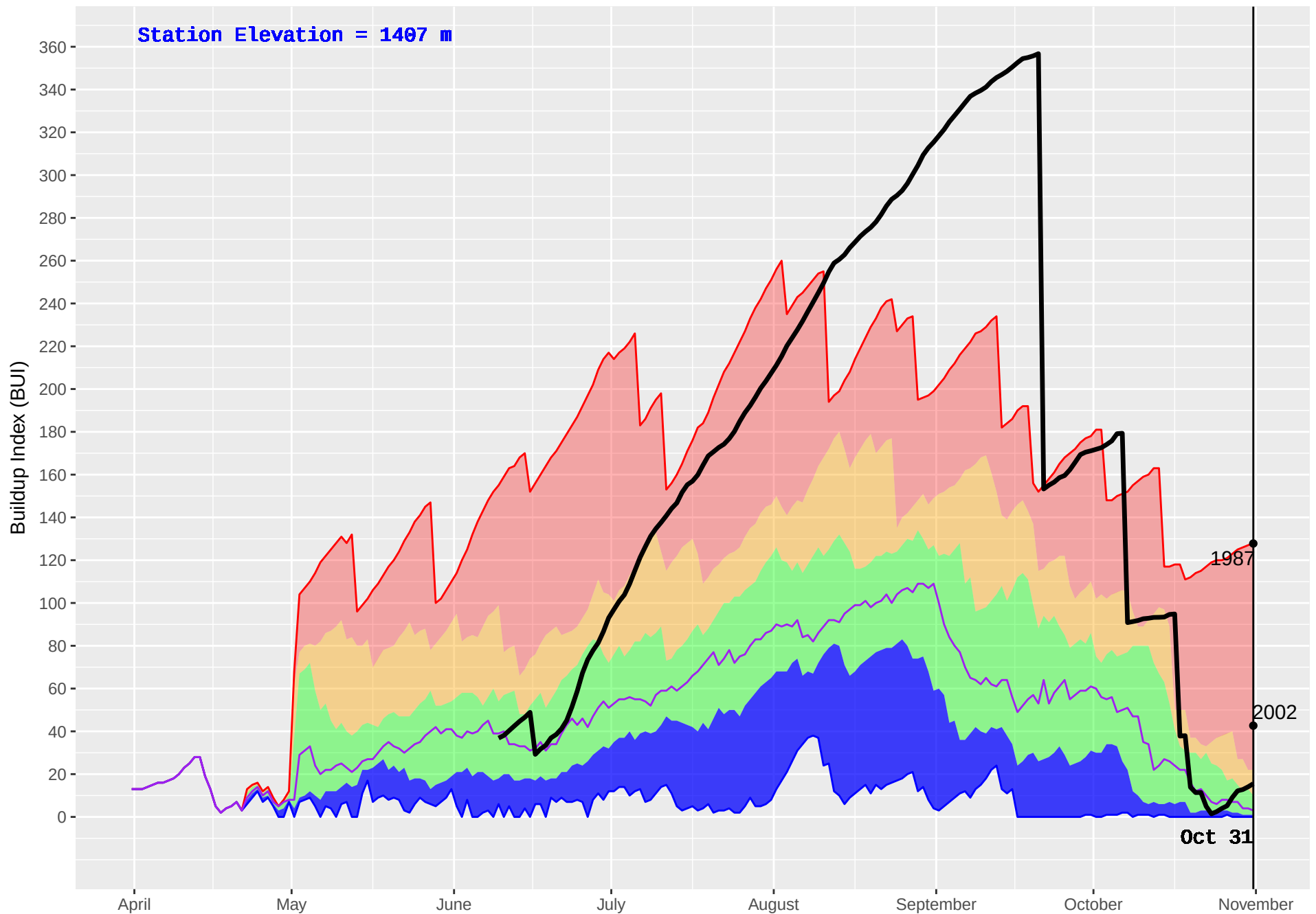
THYNNE (279) : Historical (1977–2016) and Current (2017) Noon Buildup Index (BUI)
